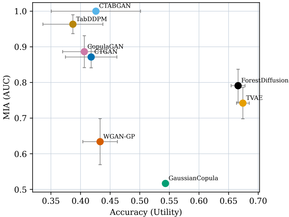
Forest Cover: Accuracy (Utility) vs MIA (AUC)
